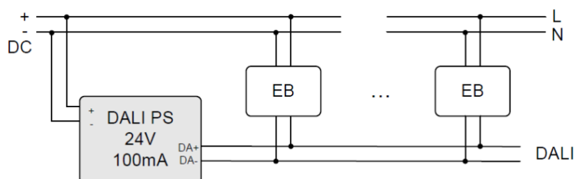
wiring diagram
