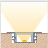
Montage in Holz- und Laminatböden integration into parquet and laminate floors
