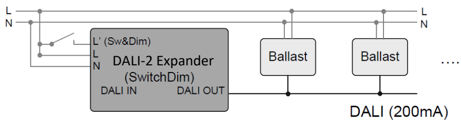
Control of DALI-ballasts via Switch-Dim (DALI-2 Expander DES)
