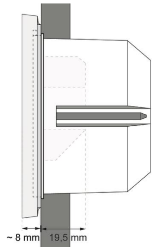
installed Touchpanel
